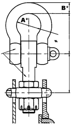
E305H Grillete
